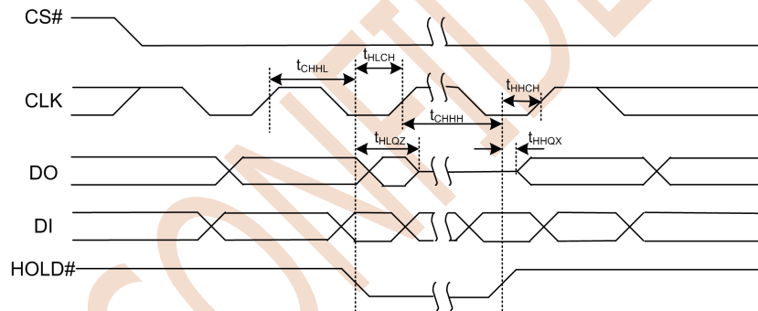
Figure 8.6 Hold Timing
