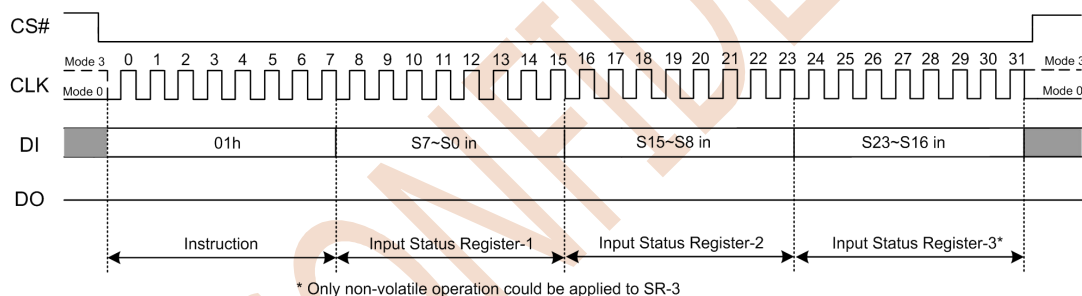
Figure 7.5a Write Status Register Instruction(SPI Mode)
