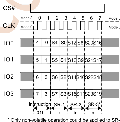
Figure 7.5b Write Status Register Instruction(QPI Mode)
